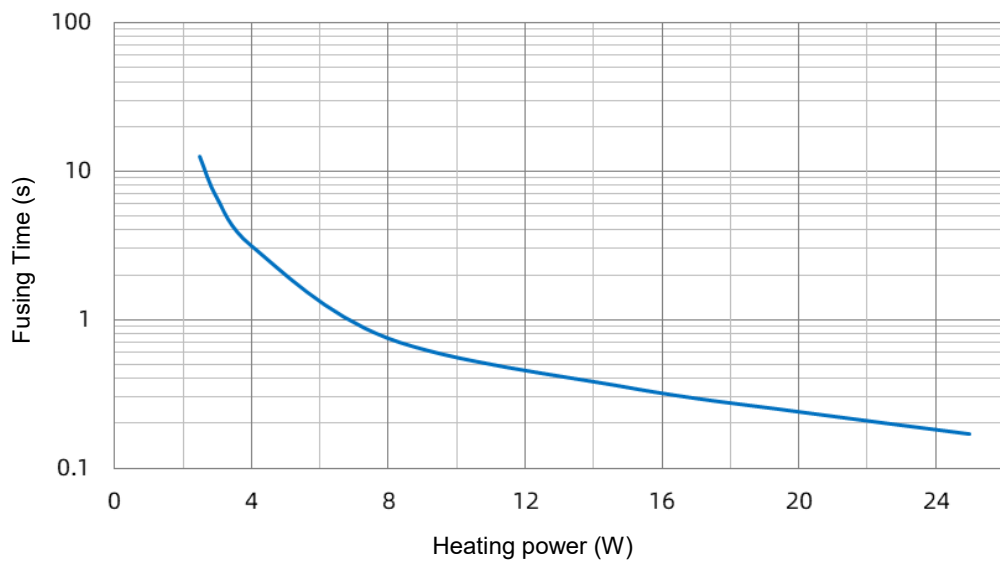
SHG 12 A Power-Time Curve
