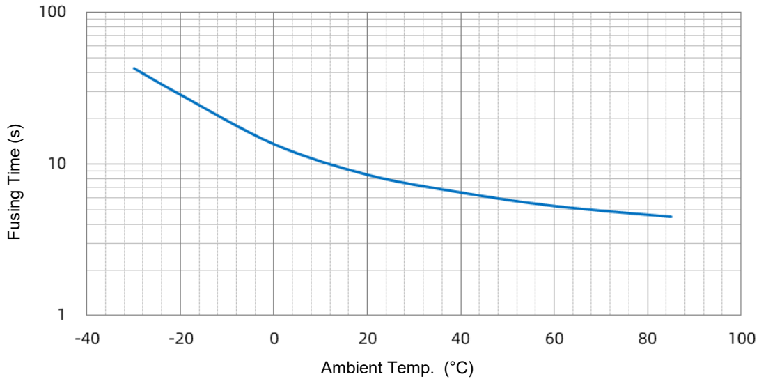
SHG 05 A Temp.-Time Curve
